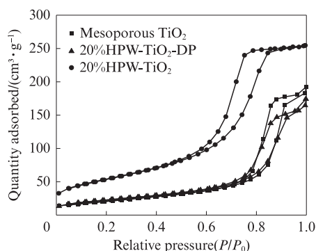
(a) N 2 adsorption and desorption isotherm
