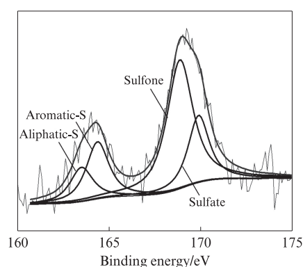
(c) S2p spectral lines of MSS with 20%HPW-TiO 2 -DP
