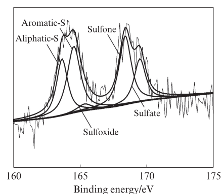
(b) S2p spectral lines of MSS
