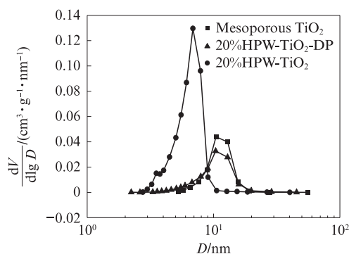
(b) BJH pore size distributions
